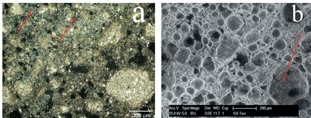
Figure 6. Microscopic features of the mortar. (a) Thin section photomicrograph (crossed nicols), showing the micritic-microsparitic texture of the binder, consisting of fine calcite mixed with hydraulic components; the aggregate is uniformly distributed within the binder and made of fragments of dolomitic limestones; (b) ESEM image, showing the high porosity of the mortar and the rounded morphology of the pores, mainly arising from air bubbles. Narrows point shrinkage microcracks that also affects the mortar structure.
