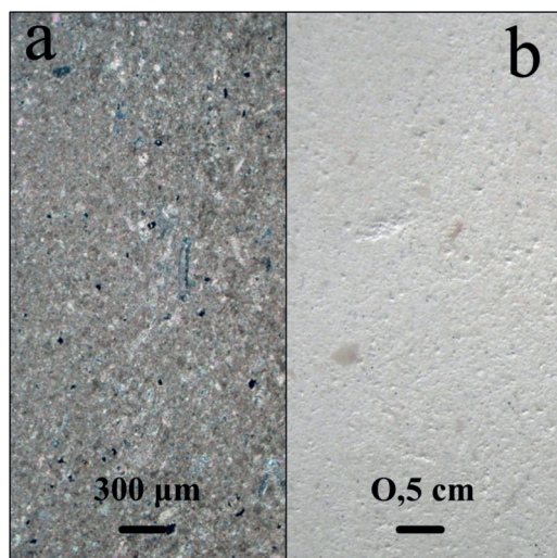
Figure 3. CS medium-fine wackestone, thin section photomicrograph, crossed nicols (a); macrophotograph (b).
