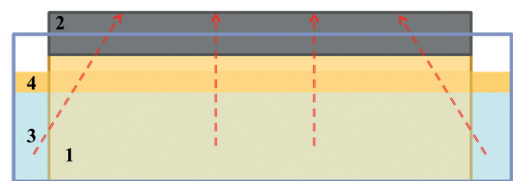
Figure 2. Experimental set-up for the evaporation test of the saline solution through the mortar/stone specimen: stone (1), mortar layer (2), saline solution (3), layer of paraffin oil (4).
