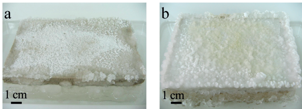
Figure 13. Efflorescences on the surface of the mortar layer applied to the CS (a) and CP (b) stones, after 4 days of the evaporation test.
