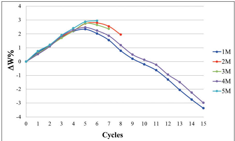
Figure 10. Weight loss of the samples during crystallization test.
