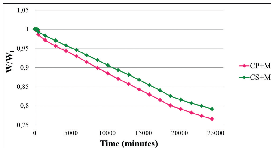
Figure 12. Evaporation rate of the saline solution through the composite specimens.
