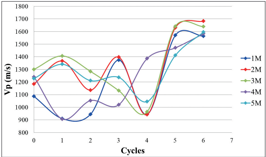
Figure 11. Velocity of the ultrasonic P-waves measured on the samples during crystallization test.
