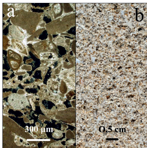
Figure 4. CP coarse grainstone, thin section photomicrograph, crossed nicols (a); macrophotograph (b).
