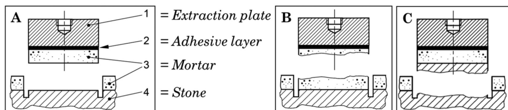
Figure 8. Different types of fractures that can occur by the adhesive strength test. A) fracture at the interface between the mortar and the support; B) fracture within the mortar; C) fracture within the support.
