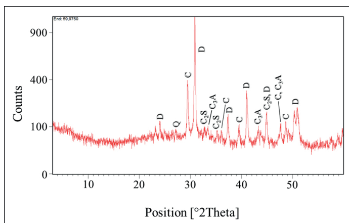
Figure 7. XRPD spectrum of the mortar (whole sample). D = dolomite; C = calcite; C_2S = dicalcium silicate; C_3A = tricalcium aluminate; Q = quartz.
