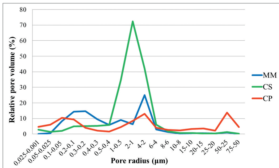
Figure 5. Pore size distributions within mortar, CP and CS stones. MM = investigated mortar.
