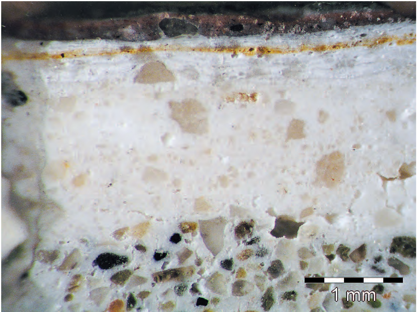
Paint stratigraphy above plaster (cross section), Kerša Palace, Dubrovnik (Croatia), 18/19th century; Photo: 2002, HRZ (Marijana Fabecić)
